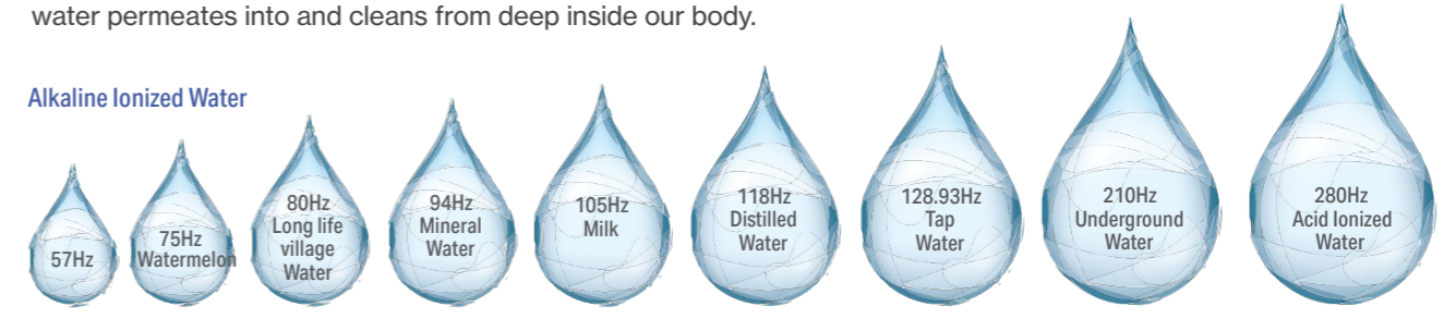
[ The size of the water molecule cluster can be measured by NMR ]
